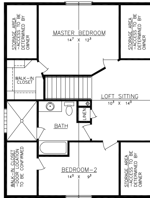
SECOND FLOOR AREA = 673 S.F.
